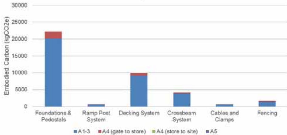
Embodied Carbon per Bridge Part, Suspended Bridge - 80m Span
