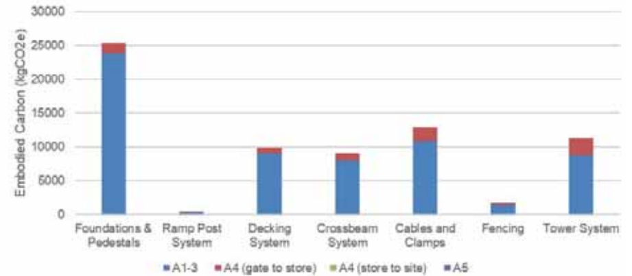
Embodied Carbon per Bridge Part, Suspension Bridge - 80m Span
